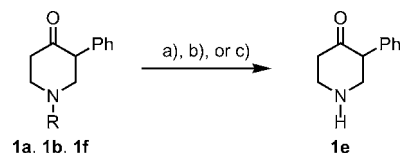
Scheme 5. N -Deprotection yielding compound 1e . For reagents and conditions see Table 4.
