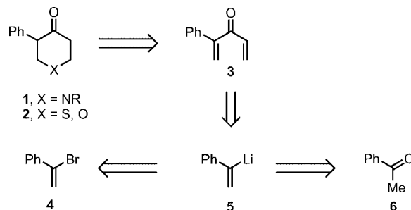
Scheme 1. Divinyl ketone 3 is accessed via \alpha -lithiostyrene ( 5 ) from either \alpha -bromostyrene ( 4 ) or more conveniently from acetophenone ( 6 ), the latter by Shapiro reaction. Compound 3 is the key building block for the preparation of 3-aryl-substituted heterocyclic ketones 1 and 2 .
