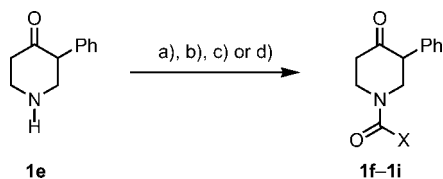
Scheme 4. N -Functionalization of piperidone 1e . For reagents and conditions see Table 3.
