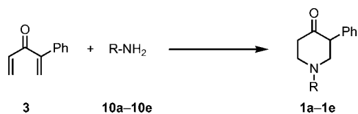
Scheme 3. Ring closure of divinyl ketone 3 with amines 10 forming 3-aryl-4-piperidones 1 . For substituents R, conditions and yields see Table 2.
